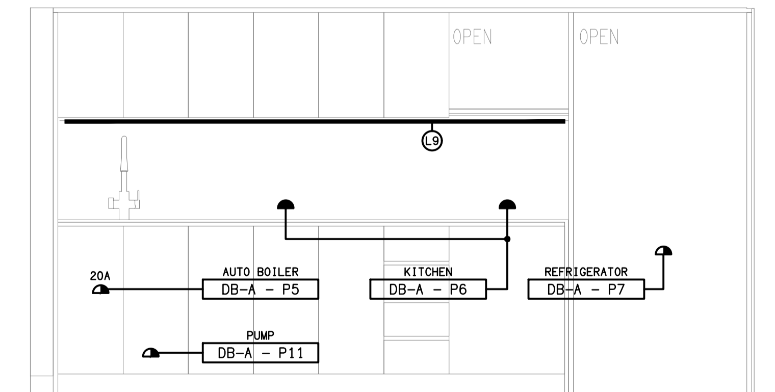
DETAIL A KITCHENETTE ELEVATION SCALE 1:20
